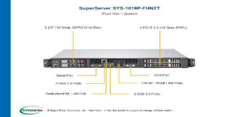
1U, 19" Rack-mount server (<450 mm wide) Indoor IT Rack
